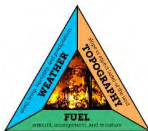
Figure 1) Fire Behavior Triangle (learn.weatherstem.com)
